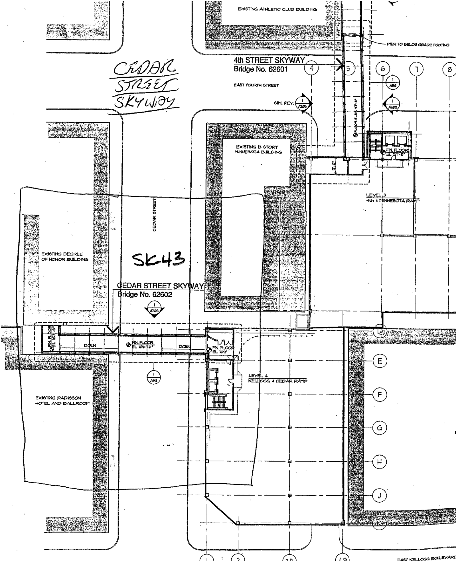
1 PLAN 1" = 20'
